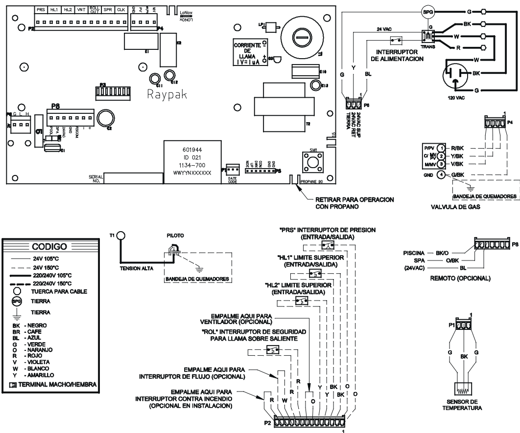
Fig. 19: Diagrama Electronico - P-D106A-AN / P-D106A-AP
