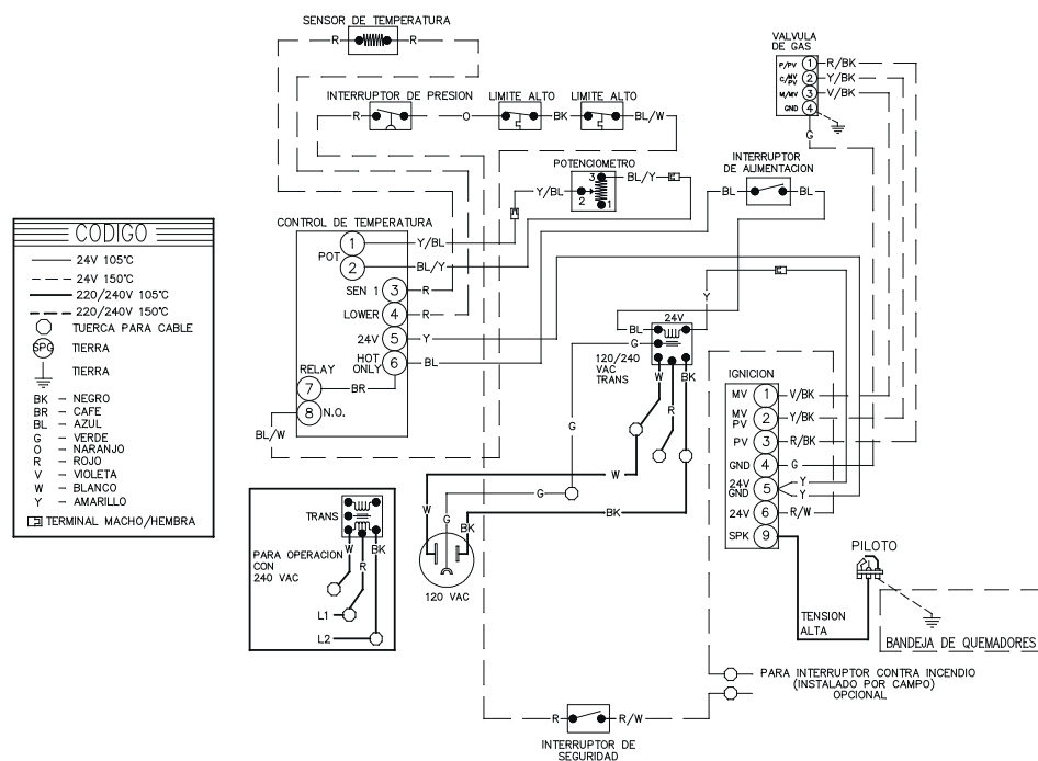
Fig. 19: Diagrama Electronico - P-D106A-AN / P-D106A-AP
