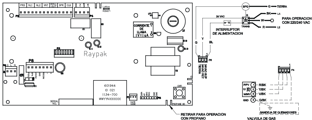
Fig. 20: Diagrama Electronico - P-D156A-EN / P-D156A-EP
